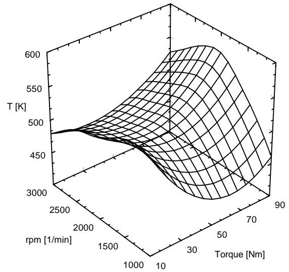
Figure 7 - Mean wall temperature as function of torque and engine speed.
